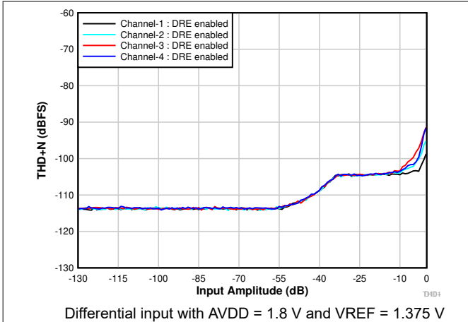
Figure 6-9. THD+N vs Input Amplitude With DRE Enabled
