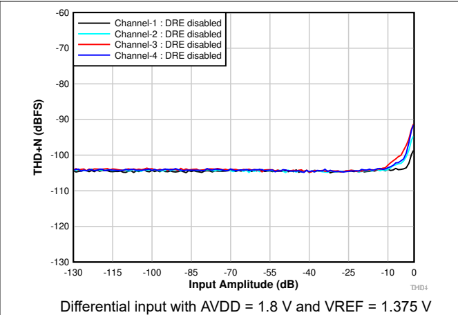
Figure 6-10. THD+N vs Input Amplitude With DRE Disabled
