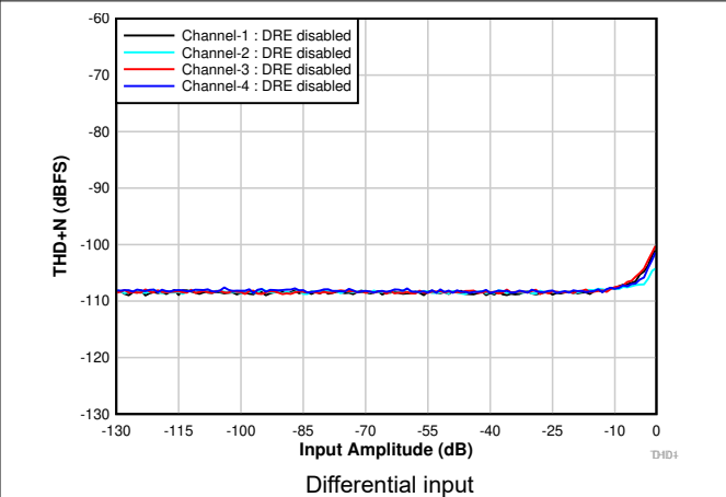
Figure 6-6. THD+N vs Input Amplitude With DRE Disabled
