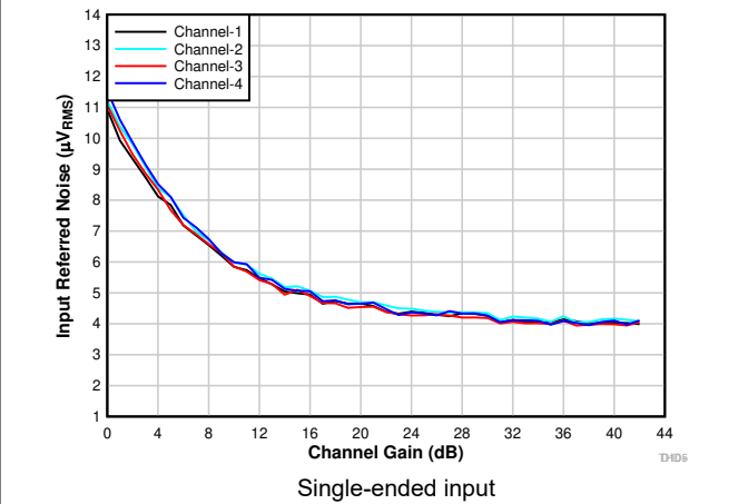
Figure 6-14. Input-Referred Noise vs Channel Gain
