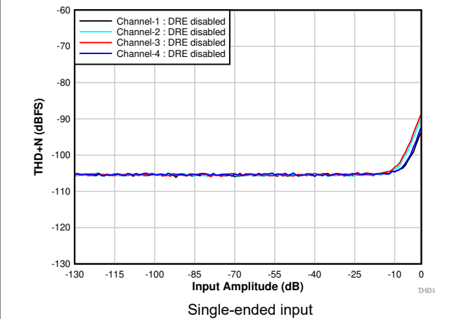
Figure 6-8. THD+N vs Input Amplitude With DRE Disabled
