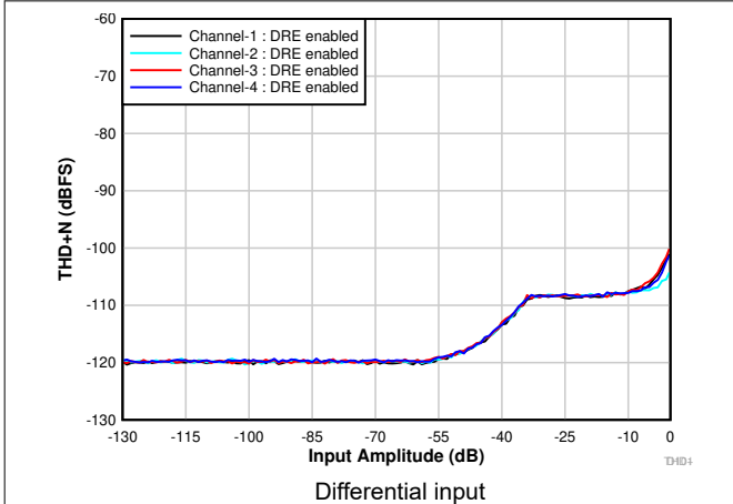
Figure 6-5. THD+N vs Input Amplitude With DRE Enabled
