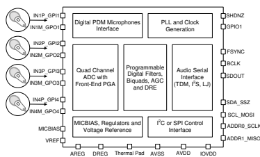
Simplified Block Diagram
