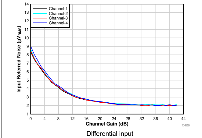
Figure 6-13. Input-Referred Noise vs Channel Gain
