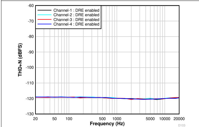
Figure 6-11. THD+N vs Input Frequency With a -60-dBr Input
