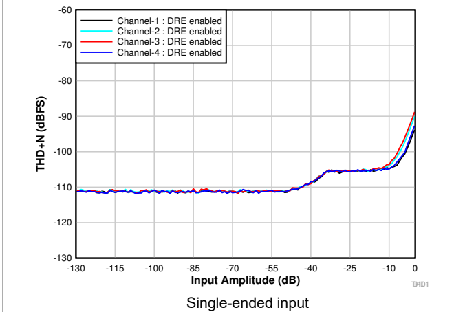
Figure 6-7. THD+N vs Input Amplitude With DRE Enabled
