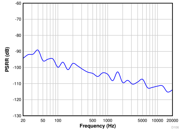
Figure 6-16. Power-Supply Rejection Ratio vs Ripple Frequency With 100-mV pp Amplitude
