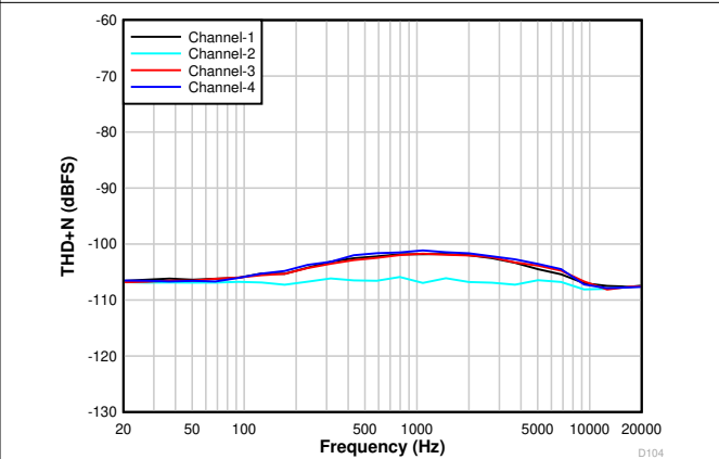
Figure 6-12. THD+N vs Input Frequency With a -1-dBr Input
