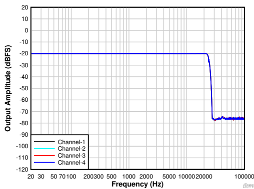
4th-order PDM modulator with PDMCLKx = 1.536\text{ MHz} Figure 6-14. Frequency Response With a -20-dBr Input
