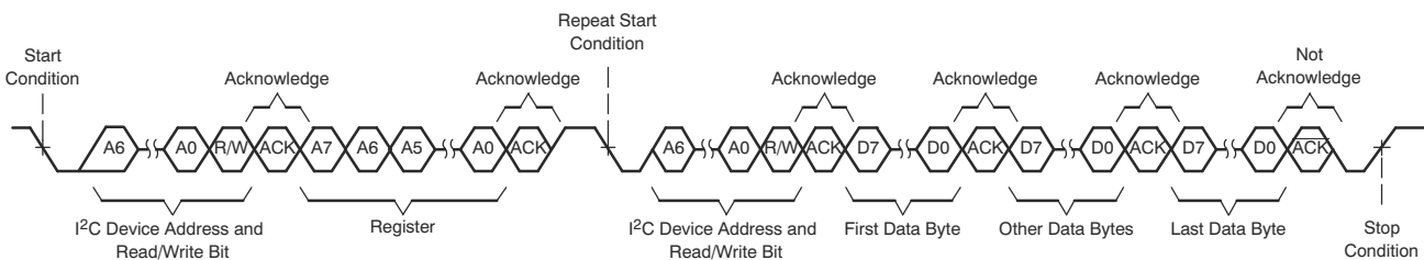
Figure 7-67. I 2 C Multiple-Byte Read Transfer
