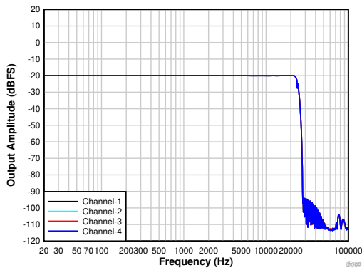
4th-order PDM modulator with PDMCLKx = 3.072\text{ MHz} Figure 6-10. Frequency Response With a -20-dBr Input
