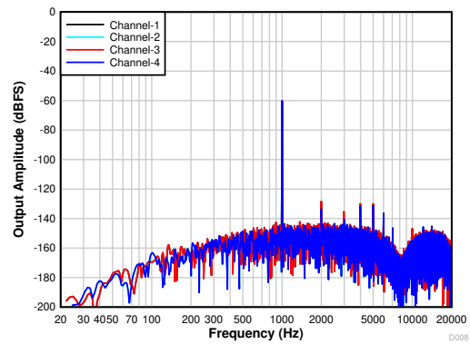
4th-order PDM modulator with PDMCLKx = 3.072\text{ MHz} Figure 6-11. FFT With a -60-dBr Input
