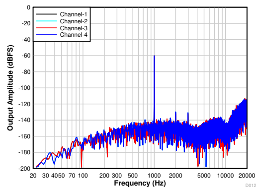
4th-order PDM modulator with PDMCLKx = 1.536\text{ MHz} Figure 6-15. FFT With a -60-dBr Input
