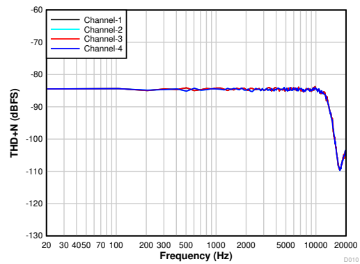
4th-order PDM modulator with PDMCLKx = 1.536\text{ MHz} Figure 6-13. THD+N vs Input Frequency With a -20-dBr Input
