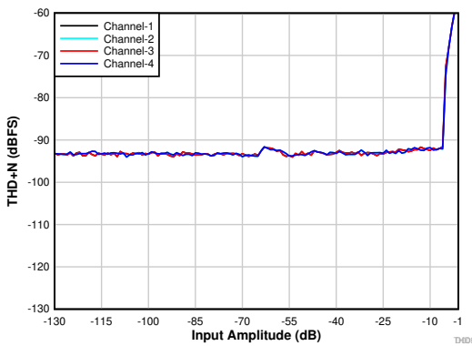
4th-order PDM modulator with PDMCLKx = 1.536\text{ MHz} Figure 6-12. THD+N vs Input Amplitude
