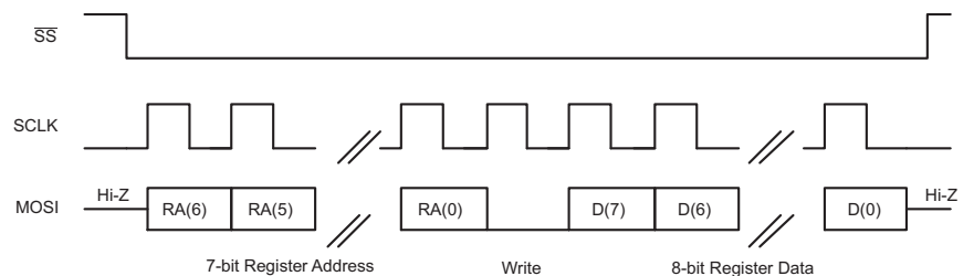
Figure 84. SPI Single-Byte Write Transfer
