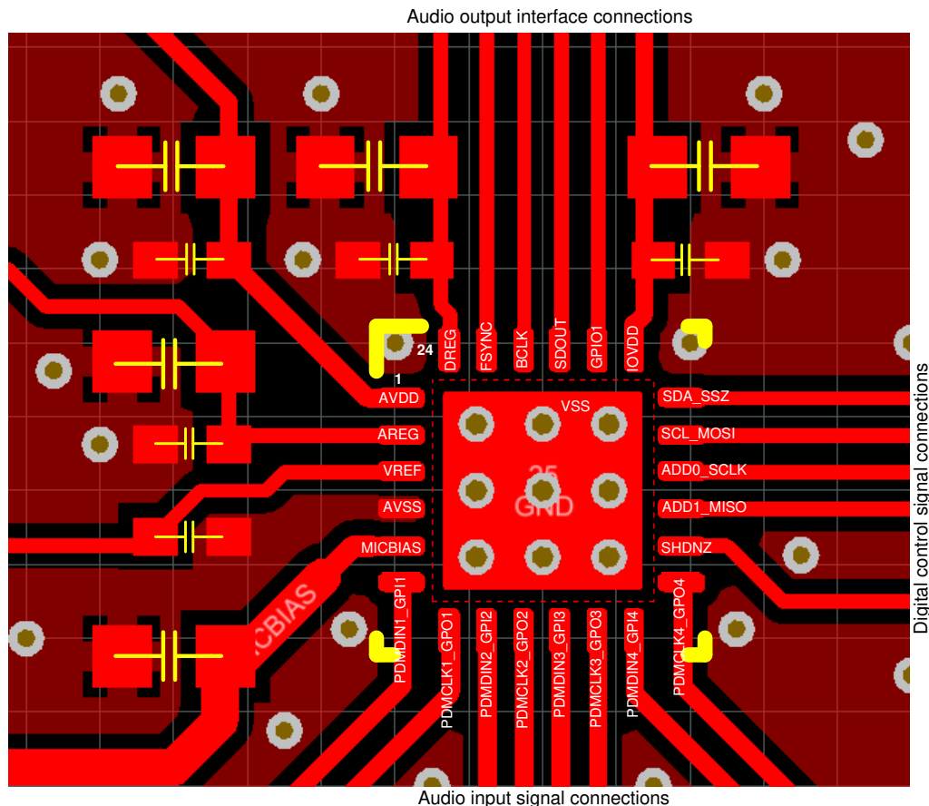
Figure 165. Layout Example
