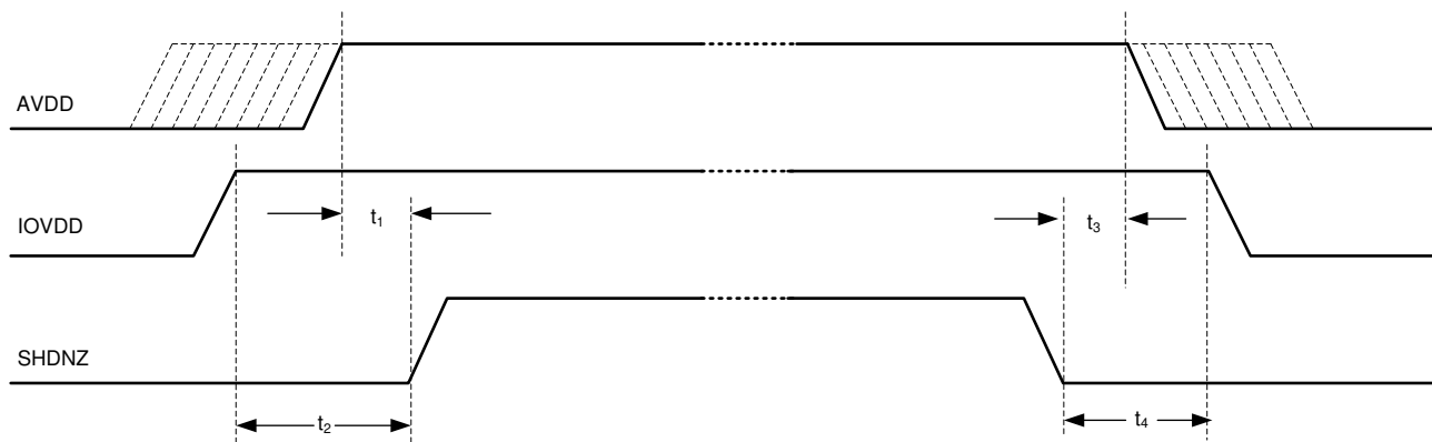
Figure 164. Power-Supply Sequencing Requirement Timing Diagram
