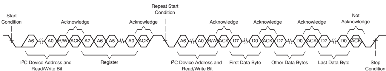
Figure 83. I 2 C Multiple-Byte Read Transfer
