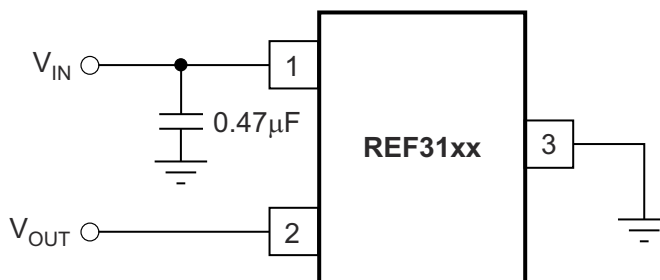
Figure 8-1. Typical Connections for Operating REF31xx
