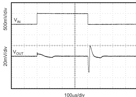
Figure 6-14. Line Transient C_L = 10\mu\text{F}
