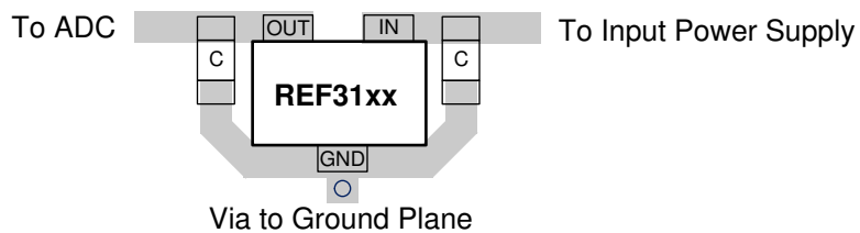
Figure 8-6. Layout Example
