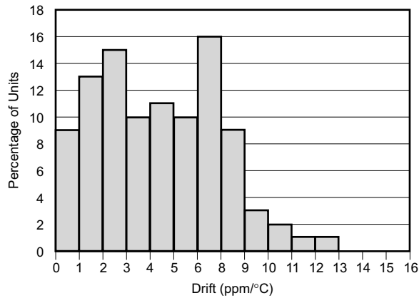
Figure 6-1. Temperature Drift (0°C to 70°C)
