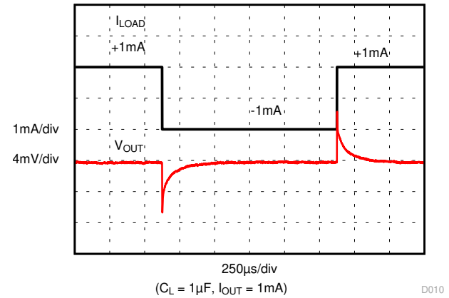
Figure 7-10. Load Transient
