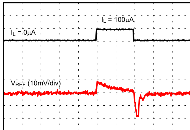
Figure 8-3. Load Transient Response 0 \mu A to 100 \mu A , C_L = 1 \mu F
