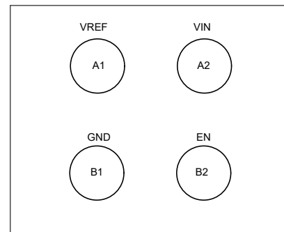
Figure 5-2. YBH Package 4-Pin WCSP Top View
