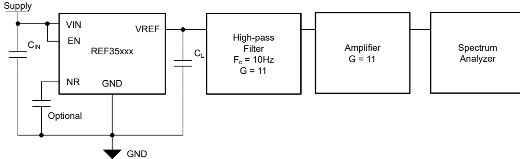
Figure 7-15. Broadband Noise Test Setup
