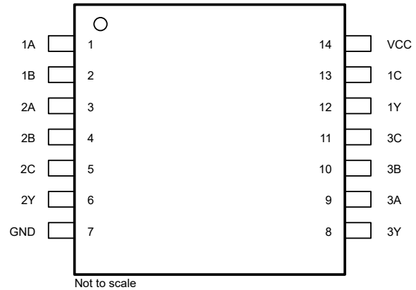
Figure 4-2. SN74LVC11A-Q1 D or PW (Preview) Packages, 14-Pin SOIC or TSSOP (Top View)
