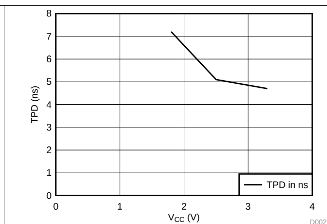
Figure 2. TPD vs V_{CC}
