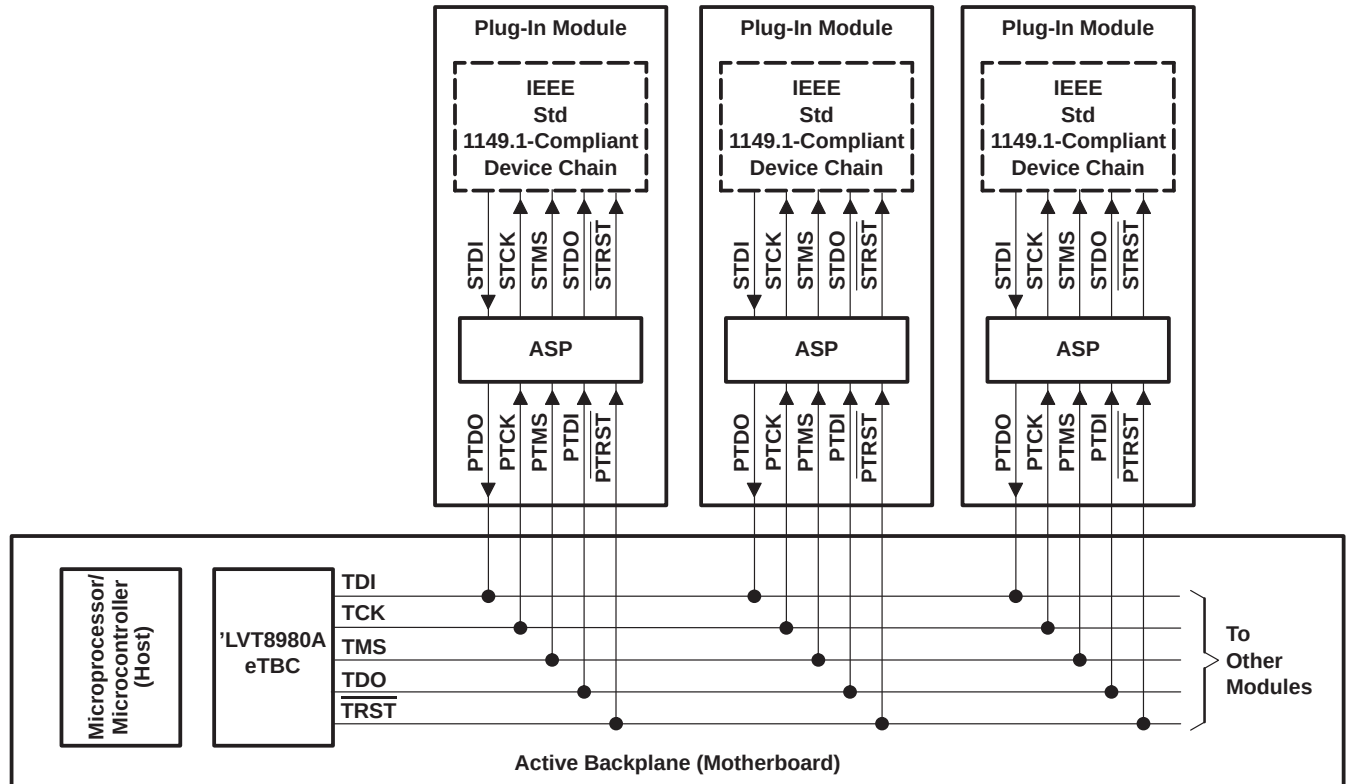
Figure 5. Active-Backplane (Motherboard) Application
