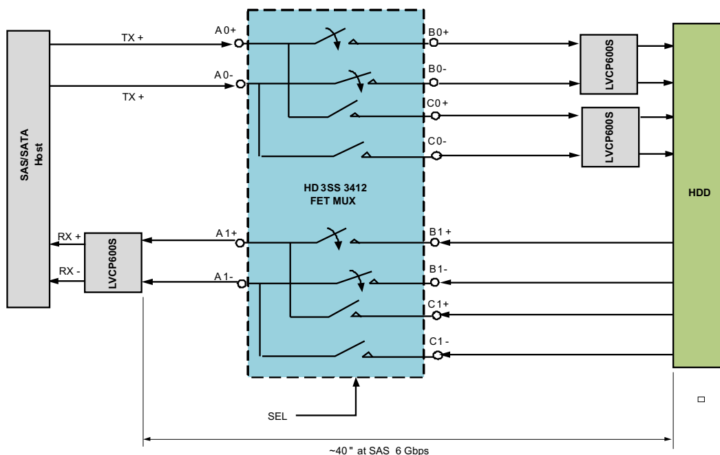
Figure 13. Typical Application
