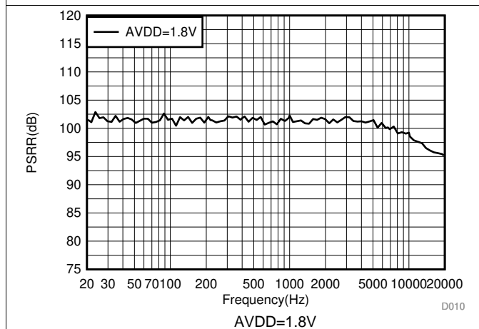
Figure 13. AVDD PSRR vs Frequency
