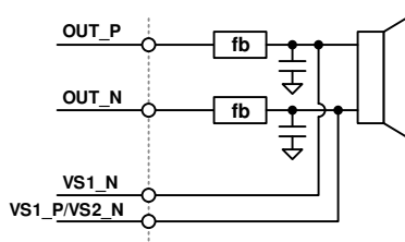
Figure 45. V-Sense Connections
