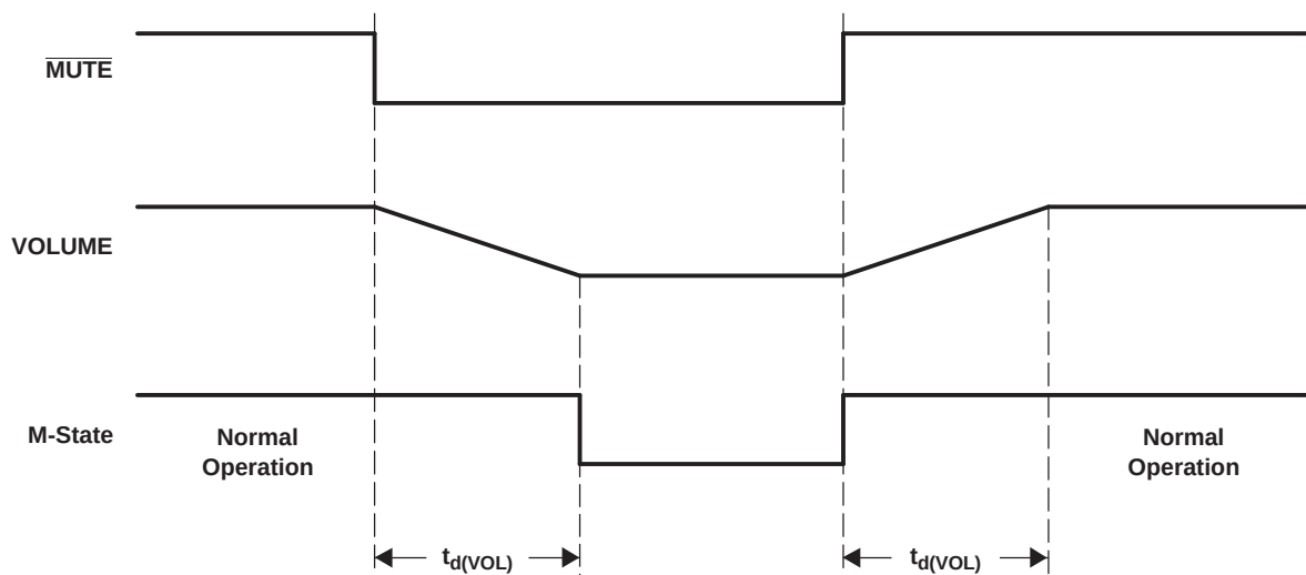
Figure 4-7. Mute Timing
