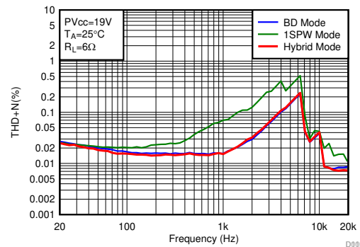
Figure 6-10. THD+N vs Frequency-BTL
