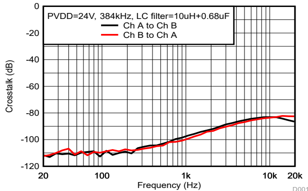
PV_{DD}=24V BD Modulation P_{out}=1W F_{sw}=384kHz Load = 6\Omega BTL Mode
