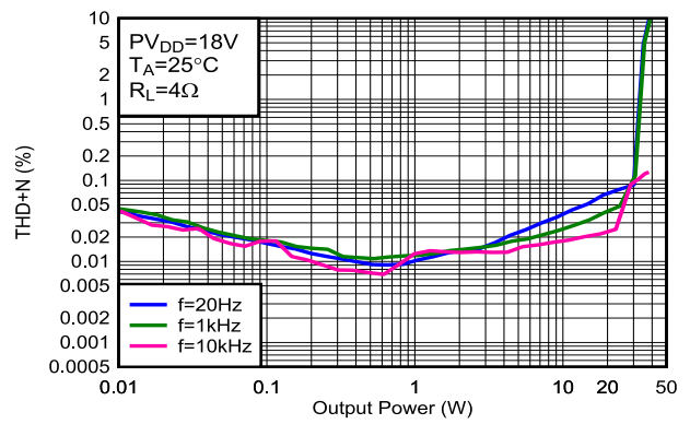
BD Modulation F_{SW}=384kHz P_{VDD} = 18V BTL Mode 120 kHz Class D Amplifier Loop Bandwidth
