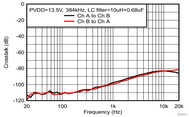
PV_{DD}=13.5V BD Modulation P_{out}=1W F_{sw}=384kHz Load = 6\Omega BTL Mode
