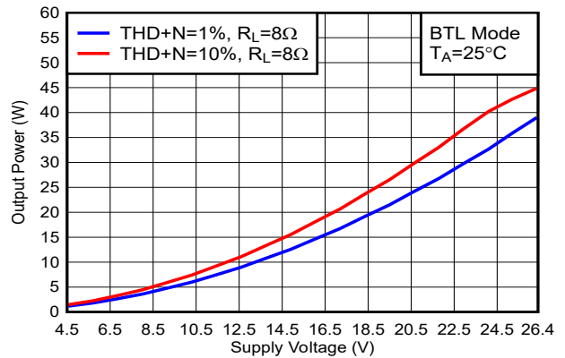
Figure 6-30. Output Power vs Supply Voltage
