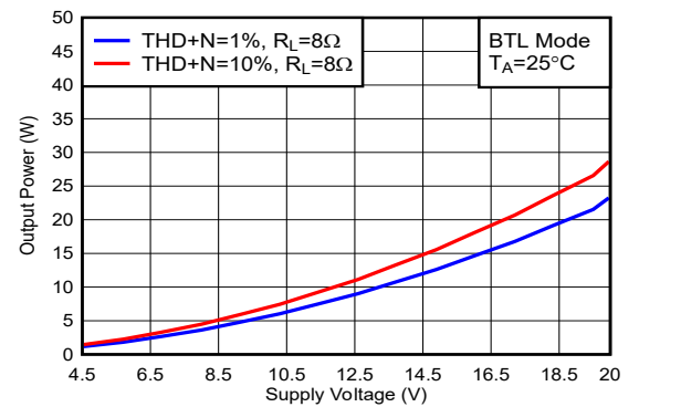
Figure 6-31. Output Power vs Supply Voltage
