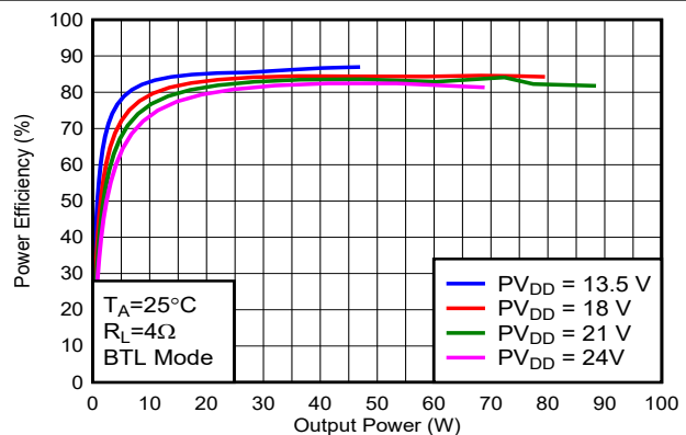
BD Modulation Load = 4\Omega BTL Mode F_{sw}=384kHz 120 kHz Class D Amplifier Loop Bandwidth
