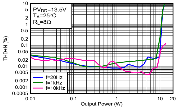
Figure 6-29. THD+N vs Output Power
