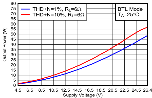
Figure 6-31. Output Power vs Supply Voltage
