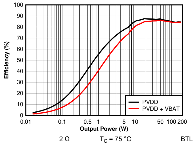
Figure 7-26. Efficiency vs Output Power - 2 \Omega - 384 kHz (Zoomed)
