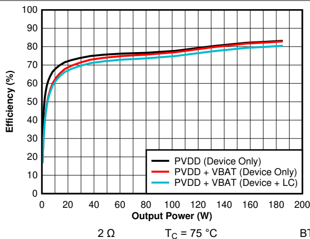
Figure 7-9. Efficiency vs Output Power - 14.4 V - 2 \Omega
