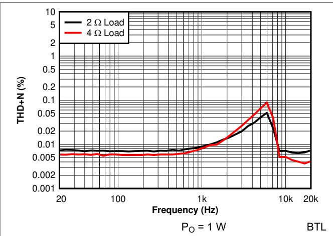
Figure 7-20. THD+N vs Frequency - 384 kHz
