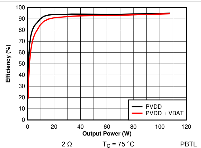
Figure 7-40. Efficiency vs Output Power - PBTL - 2 \Omega - 384 kHz
