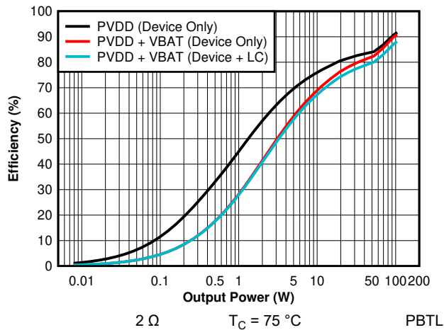
Figure 7-34. Efficiency vs Output power - PBTL - 2 \Omega (Zoomed)
