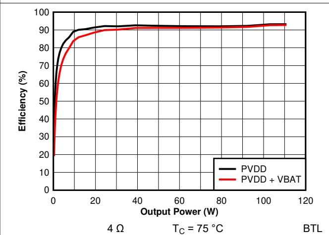
Figure 7-22. Efficiency vs Output Power - 4 \Omega - 384 kHz
