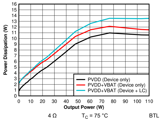
Figure 7-8. Power Dissipation vs Output Power - 14.4 V - 4 \Omega
