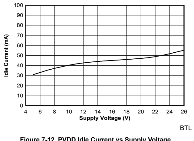
Figure 7-12. PVDD Idle Current vs Supply Voltage
