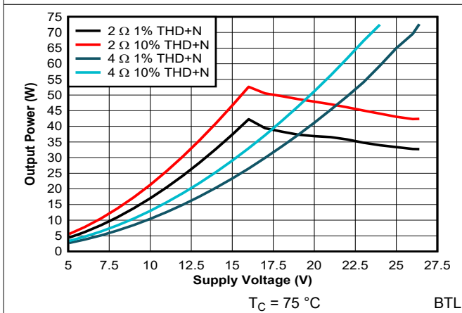
Figure 7-21. Output Power vs Supply Voltage - 384 kHz
