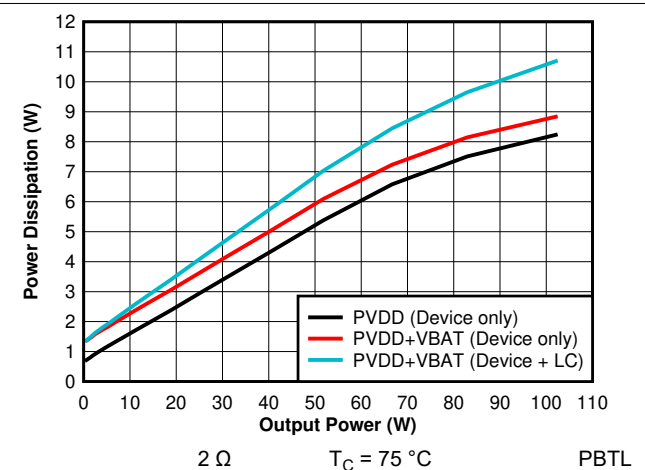
Figure 7-42. Power Dissipation vs Output Power - PBTL - 2 \Omega - 384kHz
