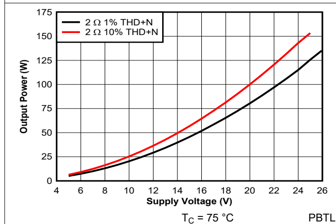
Figure 7-39. Output Power vs Supply Voltage - PBTL - 384 kHz
