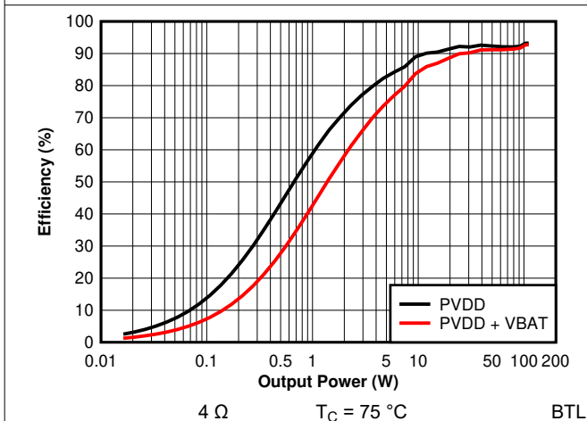
Figure 7-23. Efficiency vs Output Power - 4 \Omega - 384 kHz (Zoomed)
