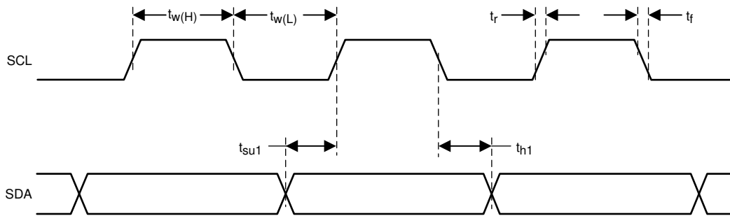
Figure 9-9. SCL and SDA Timing
