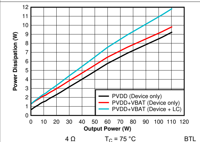
Figure 7-24. Power Dissipation vs Output Power - 4 \Omega - 384 kHz
