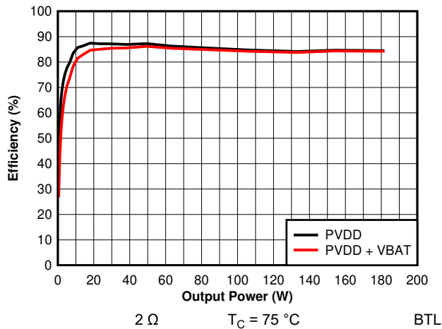
Figure 7-25. Efficiency vs Output Power - 2 \Omega - 384 kHz
