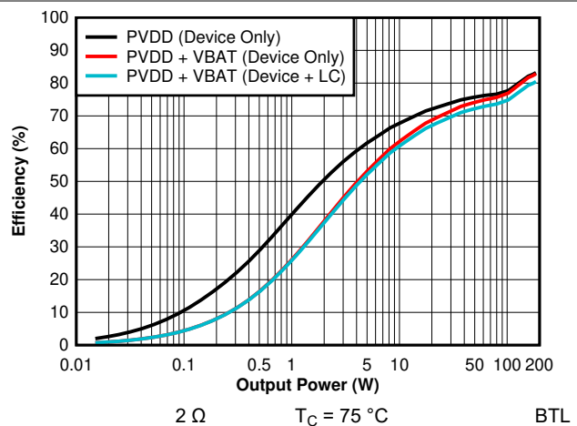
Figure 7-10. Efficiency vs Output Power - 14.4 V - 2 \Omega (Zoomed)
