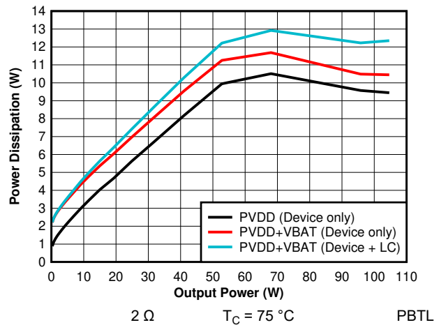
Figure 7-35. Power Dissipation vs Output Power - PBTL - 2 \Omega
