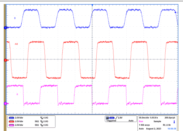
Figure 8-7. Waveforms at 20 Mbps , V_{CC} = 5\text{ V}
