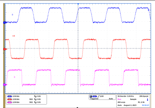
Figure 8-9. Waveforms at 20 Mbps , V_{CC} = 3.3\text{ V}
