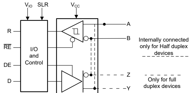
Figure 7-1. THVD2410 and THVD2450 Block Diagram
