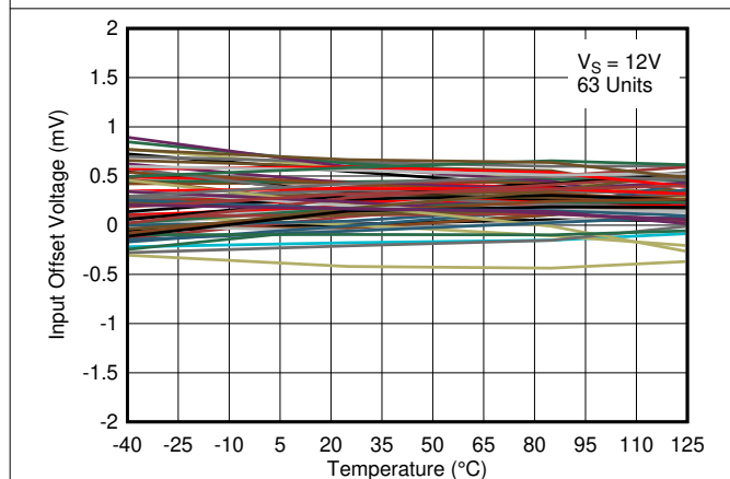
Figure 5-17. Input Offset Voltage vs. Temperature at 12V
