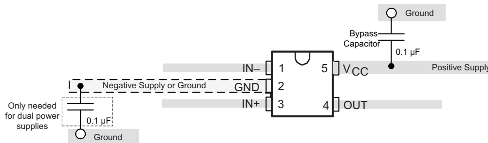
Figure 8-4. TL331-Q1 Layout Example
