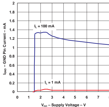
Figure 14. Ground Current vs Supply Voltage
