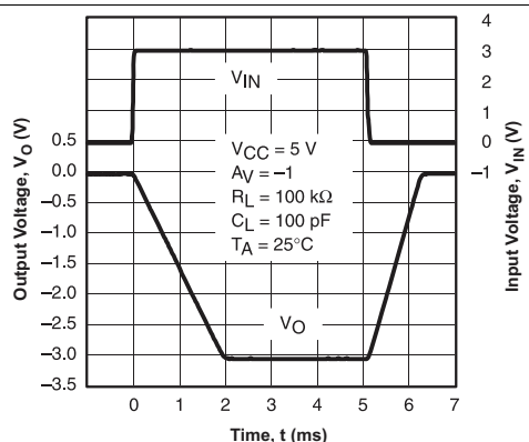
Figure 33. Large Signal Follower Pulse Response
