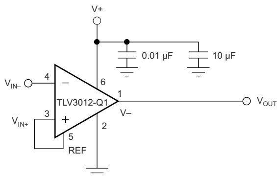
Figure 10-1. Basic Connections
