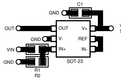
Figure 10-7. Layout Example
