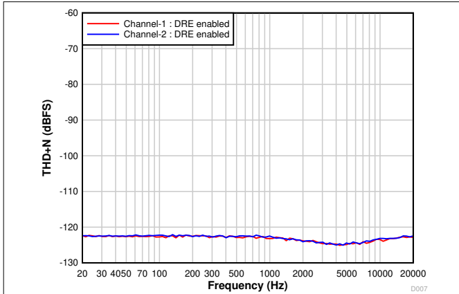
Figure 7-10. THD+N vs Input Frequency at -60-dBr Input With DRE Enabled
