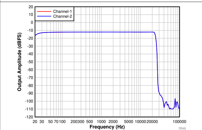
Figure 7-15. Frequency Response With a -12-dBr Input
