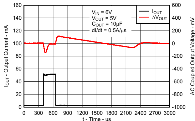
Figure 8-8. Load Transient Response for New Chip
