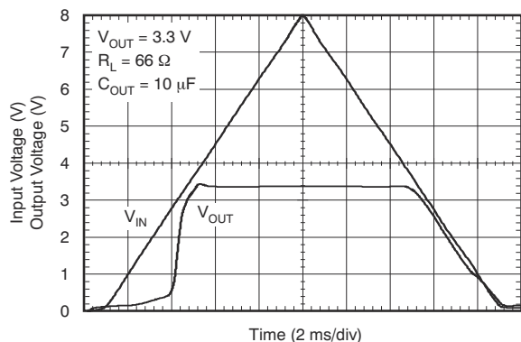
Figure 8-3. Power-Up, Power-Down for Legacy Chip
