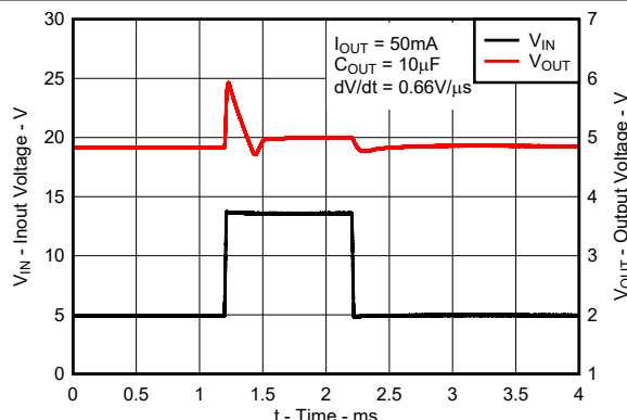
Figure 8-10. Dropout Exit Transient Response for New Chip
