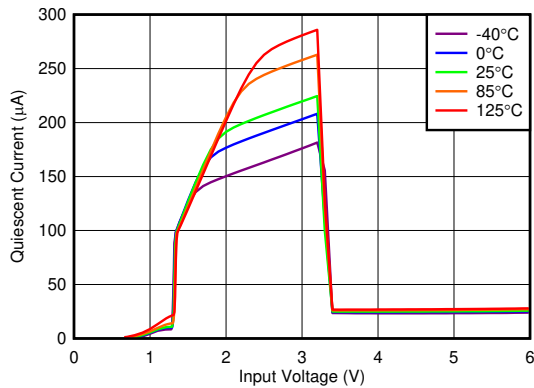
V_{OUT} = 3.3\text{V} , I_{OUT} = 0\text{mA} Figure 5-19. I_Q vs V_{IN}
