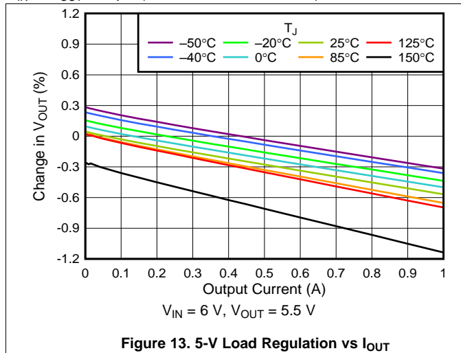
Figure 13. 5-V Load Regulation vs I_{OUT}
