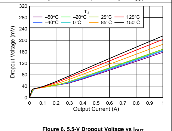
Figure 6. 5.5-V Dropout Voltage vs I_{OUT}
