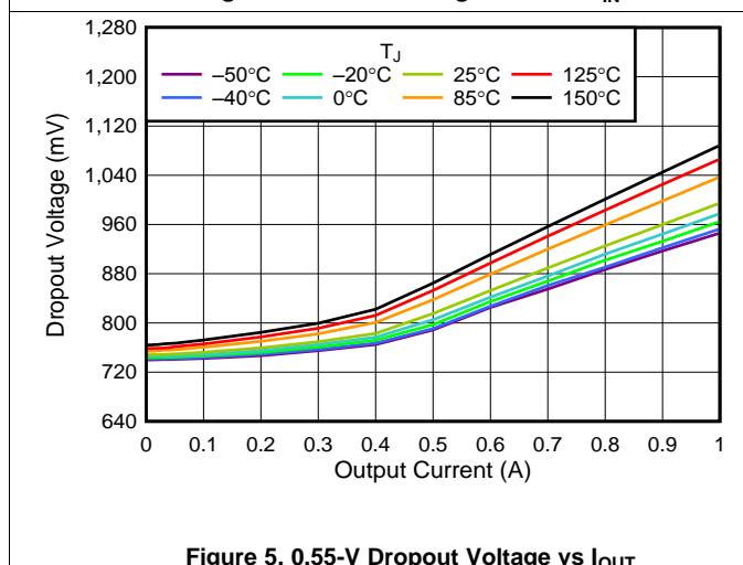
Figure 5. 0.55-V Dropout Voltage vs I_{OUT}
