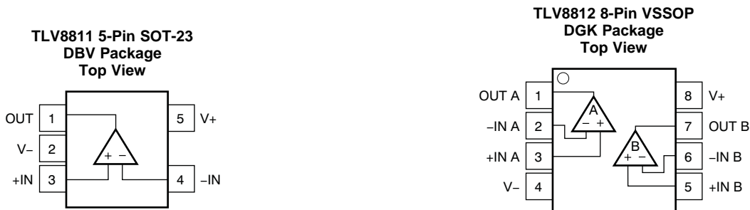
Pin Functions: TLV8811 DBV
