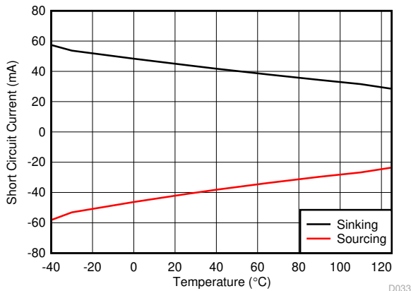
D033 Figure 6-33. Short-Circuit Current vs Temperature
