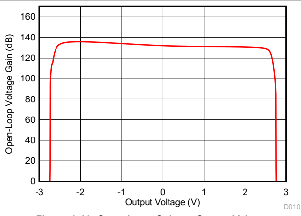
Figure 6-10. Open-Loop Voltage Gain vs Output Voltage
