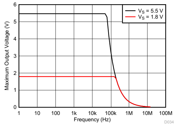
D034 Figure 6-34. Maximum Output Voltage vs Frequency
