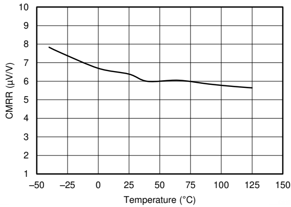
Figure 8-13. CMRR vs Temperature
