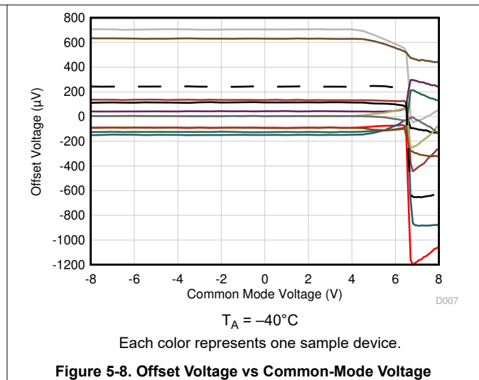
Figure 5-8. Offset Voltage vs Common-Mode Voltage
