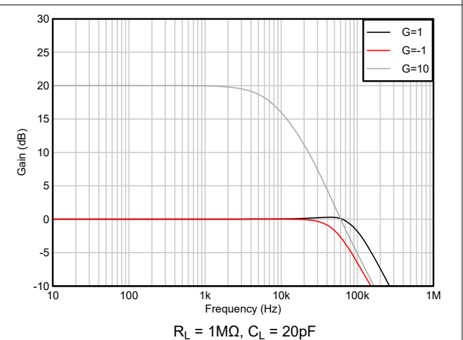
Figure 5-6. Closed-Loop Gain vs Frequency
