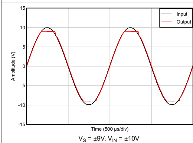
Figure 5-35. No Phase Reversal
