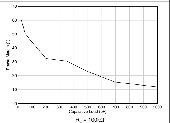
Figure 5-4. Phase Margin vs Capacitive Load
