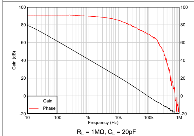
Figure 5-3. Open-Loop Gain and Phase vs Frequency
