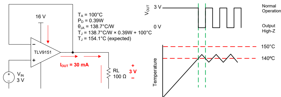
Figure 6-2. Thermal Protection
