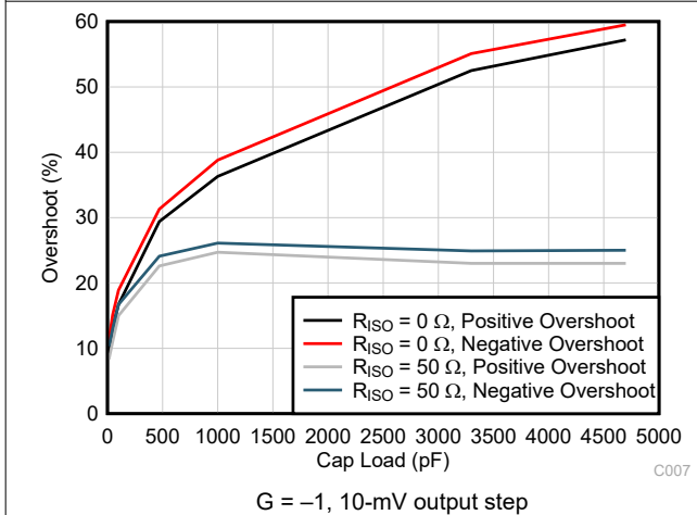
Figure 5-27. Small-Signal Overshoot vs Capacitive Load C007
