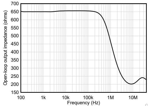
Figure 5-26. Open-Loop Output Impedance vs Frequency C013
