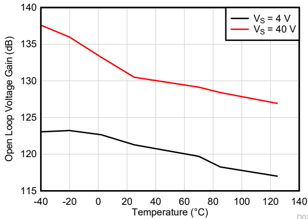
Figure 5-25. Open-Loop Voltage Gain vs Temperature (dB) D023
