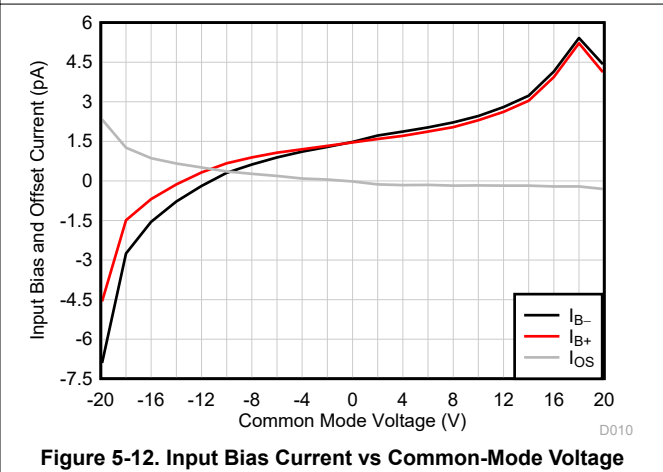
Figure 5-12. Input Bias Current vs Common-Mode Voltage
