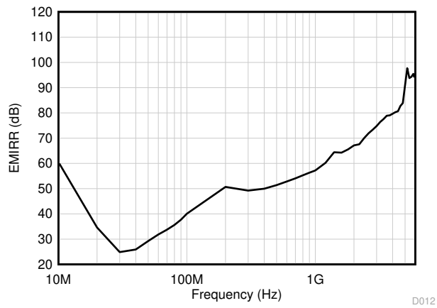
Figure 6-37. EMIRR (Electromagnetic Interference Rejection Ratio) vs Frequency D012
