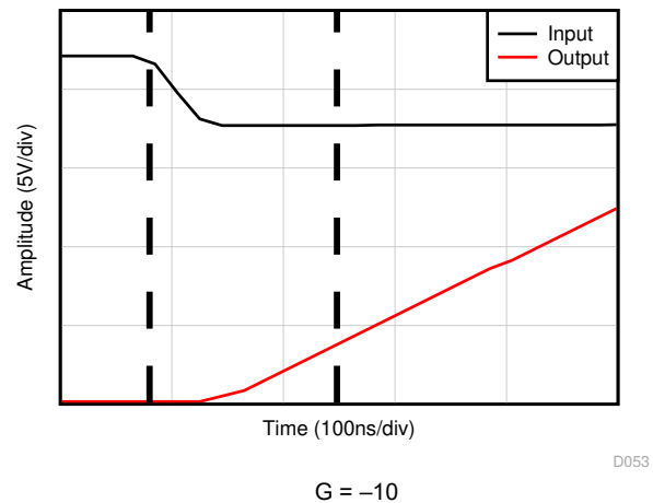
Figure 6-30. Negative Overload Recovery G = -10
