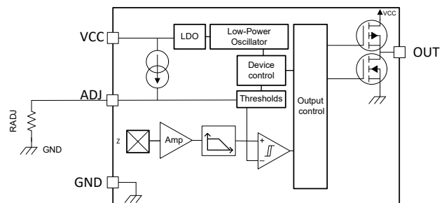
Typical Schematic
