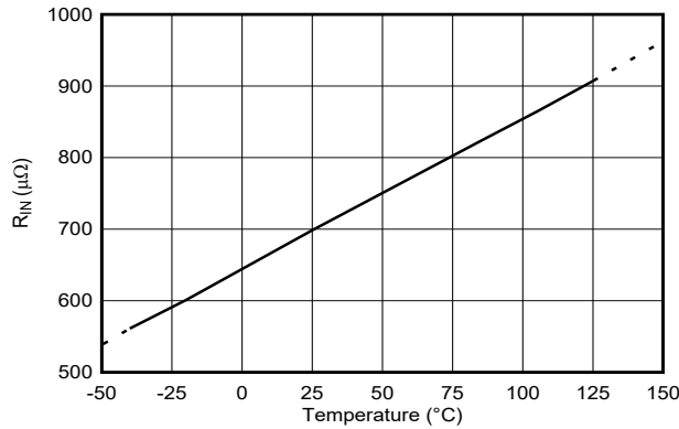
Figure 6-17. Input Conductor Resistance vs Temperature
