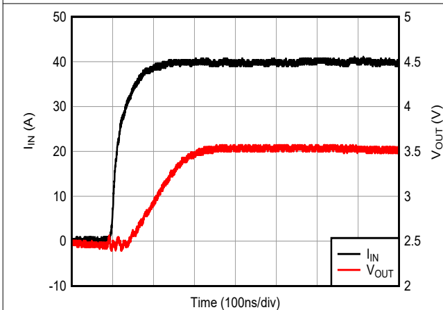
Figure 6-11. Voltage Output Step Response, Rising
