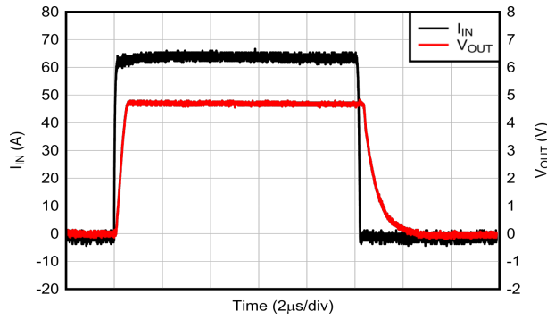
Figure 6-13. Current Overload Response
