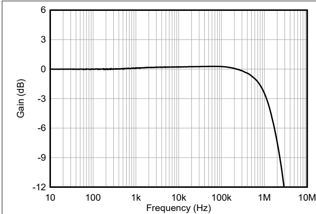
Figure 6-7. Sensitivity vs Frequency, All Gains Normalized to 1Hz
