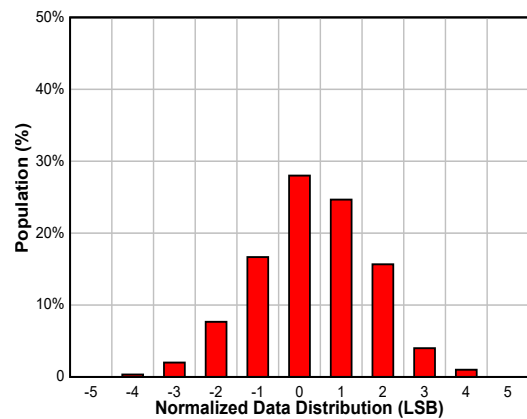
Figure 7-12. Data Distribution With 3-ms Conversion Time and Averaging On in 16-Bit Format
