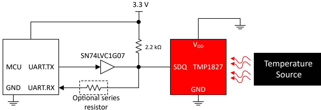
Figure 9-3. Using UART to Interface TMP1827
