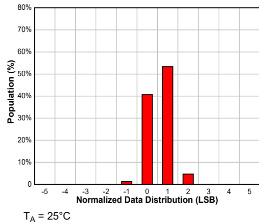
Figure 7-12. Data Distribution With 3-ms Conversion Time and Averaging On in 16-Bit Format
