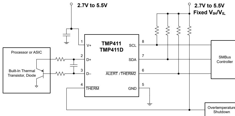
Figure 9-1. TMP411/TMP411D Simplified Block Diagram (Separate I 2 C Pullup and Supply Voltage Application while V+ \geq 2.7V )
