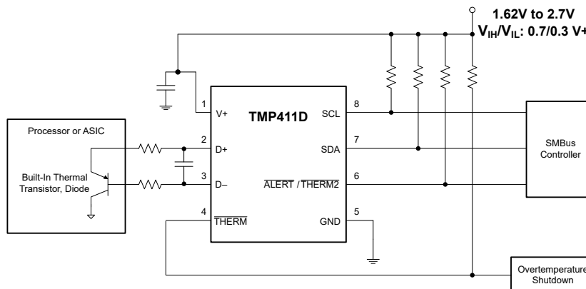
Figure 9-2. TMP411D Simplified Block Diagram (Equal I 2 C Pullup and Supply Voltage Application while V+ < 2.7V )
