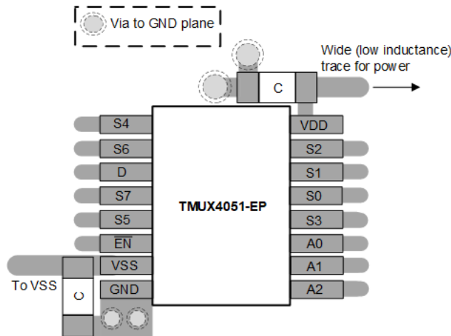
Figure 8-3. Layout Example
