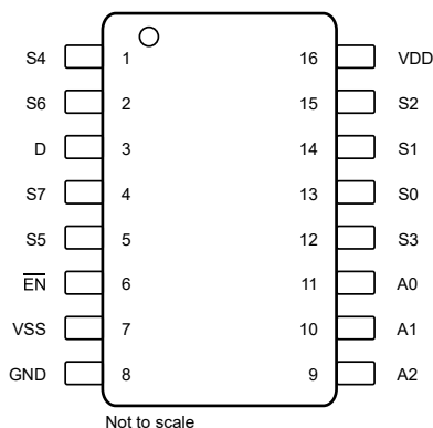
Figure 4-1. TMUX4051-EP DYY Package, 16-Pin SOT-23-THIN (Top View)
