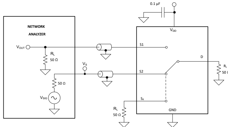
Figure 6-10. Channel-to-Channel Crosstalk Measurement Setup
