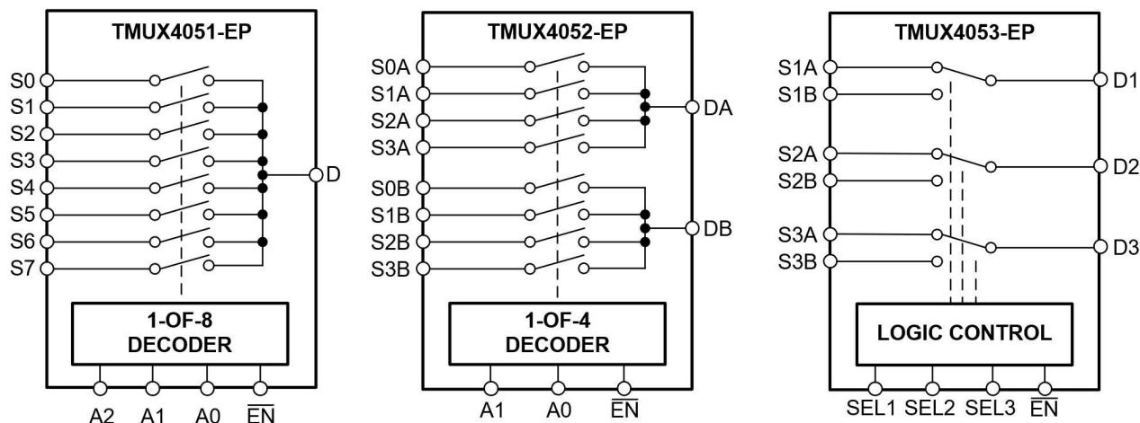
TMUX405x-EP Block Diagram
