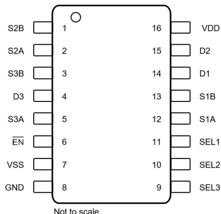
Figure 4-3. TMUX4053-EP DYY Package, 16-Pin SOT-23-THIN (Top View)
