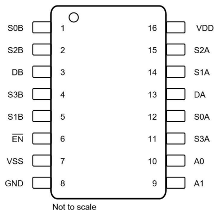
Figure 4-2. TMUX4052-EP DYY Package, 16-Pin SOT-23-THIN (Top View)
