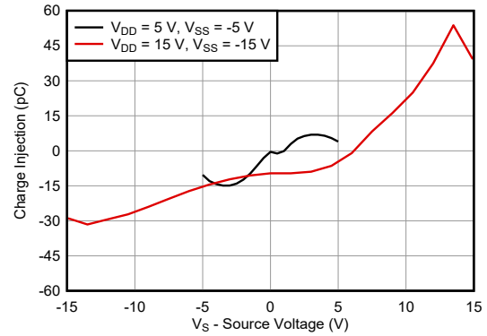
Figure 6-14. Charge Injection vs Source Voltage – Dual Supplies
