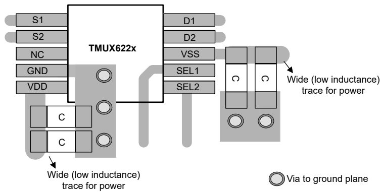
Figure 9-4. TMUX622x Layout Example
