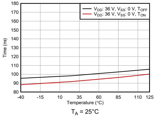
Figure 6-19. T_{ON} and T_{OFF} vs Temperature
