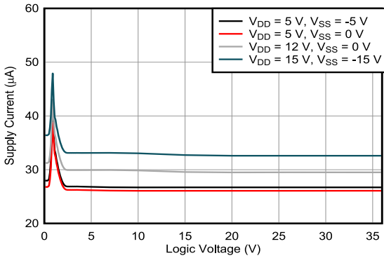
Figure 6-13. Supply Current vs Logic Voltage
