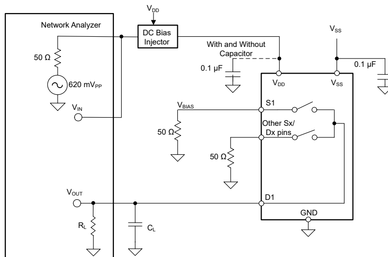
Figure 7-12. AC PSRR Measurement Setup
