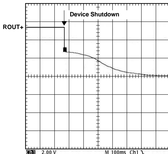
Figure 23. Shutdown Sequence in the Fade-off Mode
