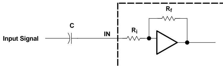
Figure 25. Resistor on Input for Cut-Off Frequency
