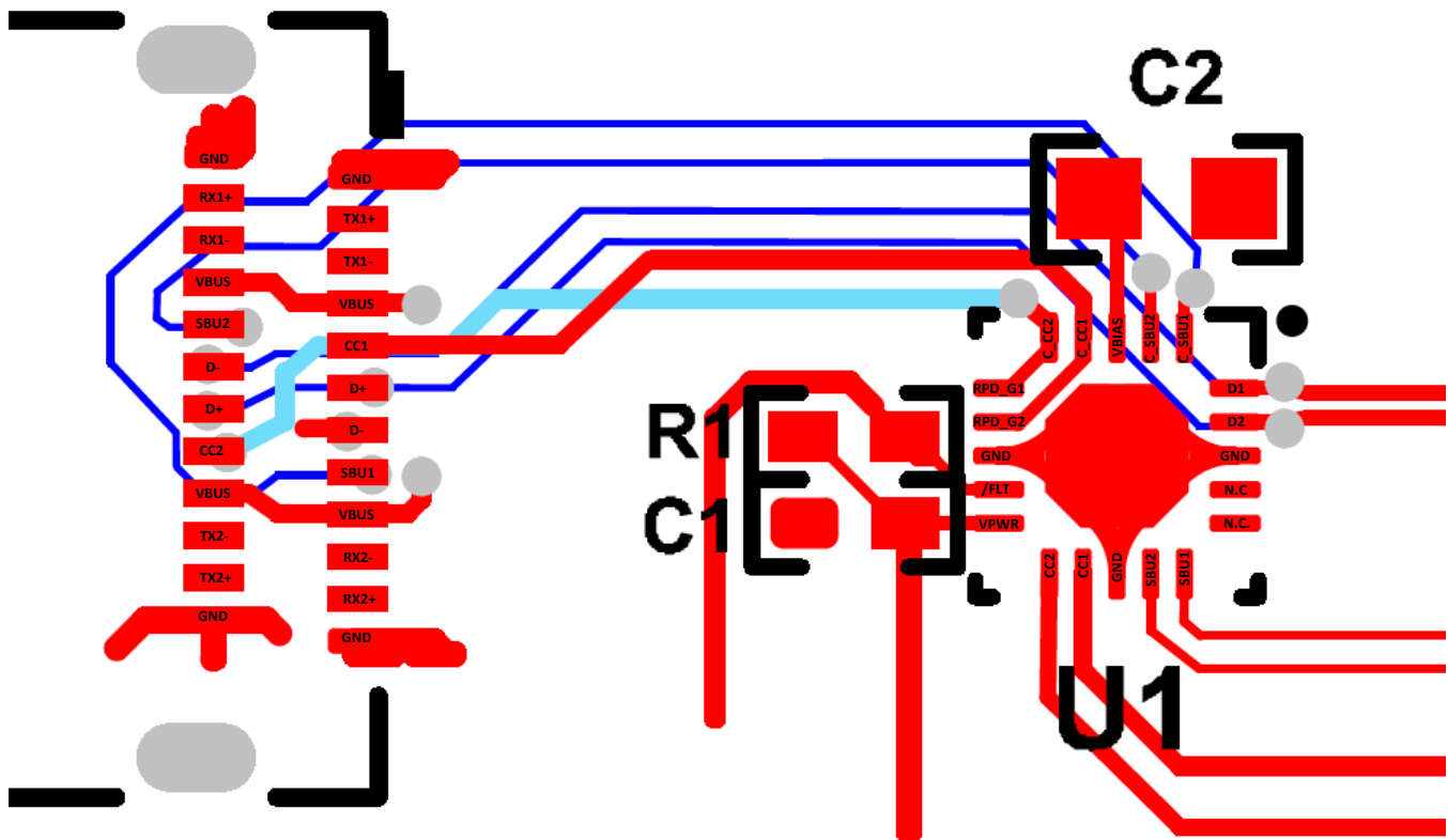
Figure 34. TPD6S300 Typical Layout
