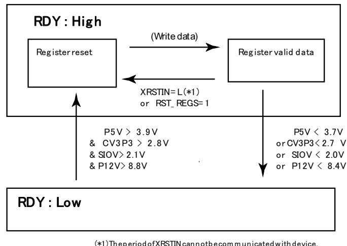
Figure 12. RDY Pin Behavior
