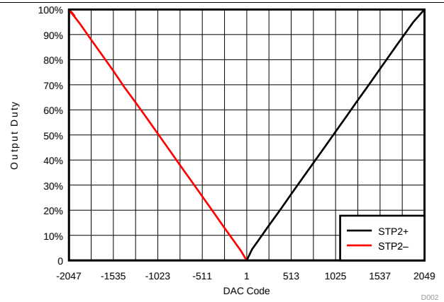
Figure 5. STP2 Driver: DAC Code vs Output On Duty
