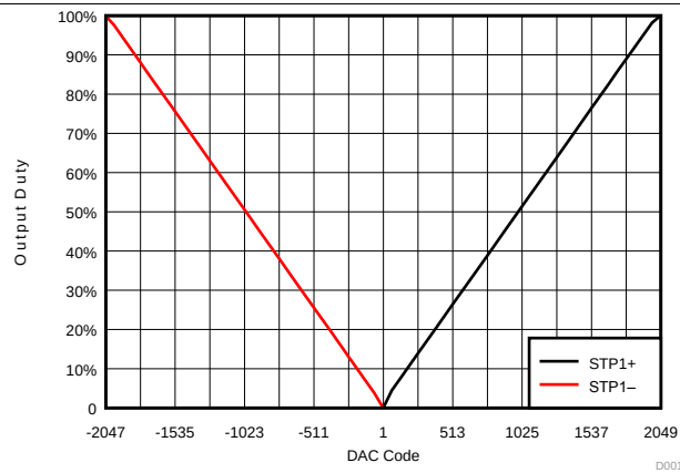
Figure 4. STP1 Driver: DAC Code vs Output On Duty
