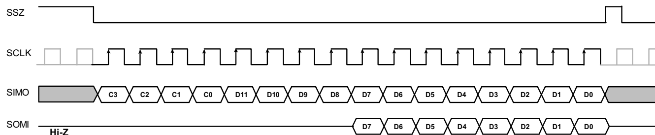
Figure 16. Write 12-Bits Focus DAC Data + Read 8-Bits Status Data
