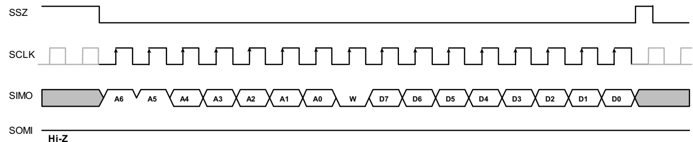
Figure 14. Write 8-Bits Control Register
