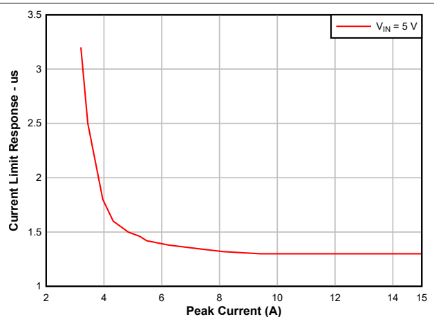
Figure 6-18. Current Limit Response ( t_{IQS} ) vs Peak Current
