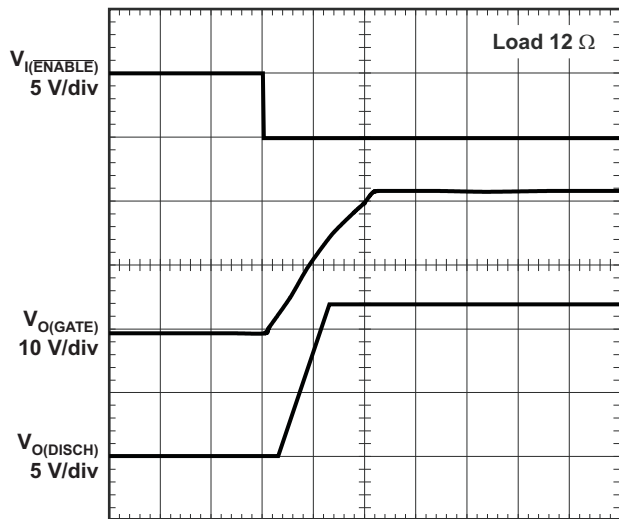
Figure 1. Turnon Voltage Transition
