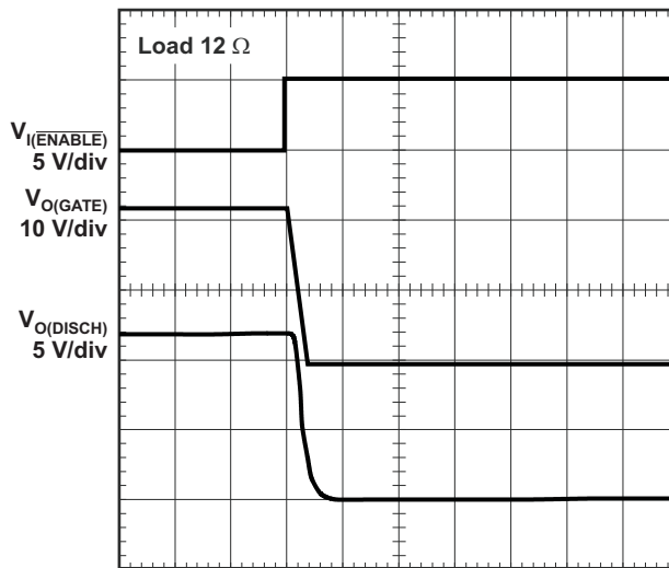
Figure 2. Turnoff Voltage Transition
