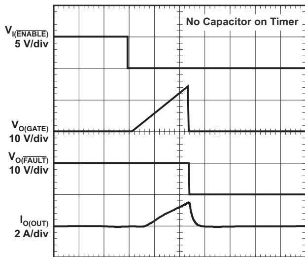
Figure 3. Overcurrent Response: Enabled Into Overcurrent Load
