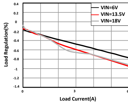
Figure 11-6. Load Regulation
