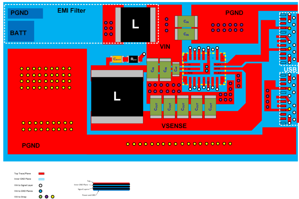
Figure 13-1. Layout Example
