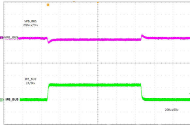
Figure 11-9. Load Transient Without Cable Compensation
