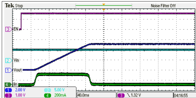
Figure 43. Output Ramp Up
